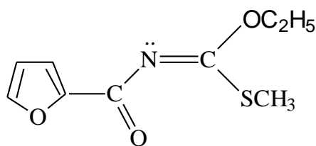
Fig.1. Estructura del N-furoyl-O-ethyl-S-methylcarbonimidetioate
