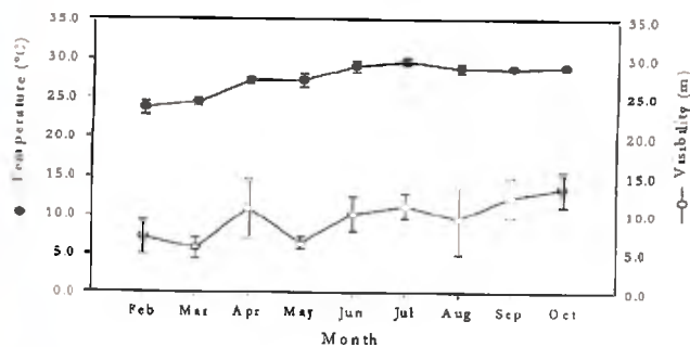
Fig. 2. Variation in temperature and visibility from February to October 1997, East of Papagayo, Guanacaste, Costa Rica.
